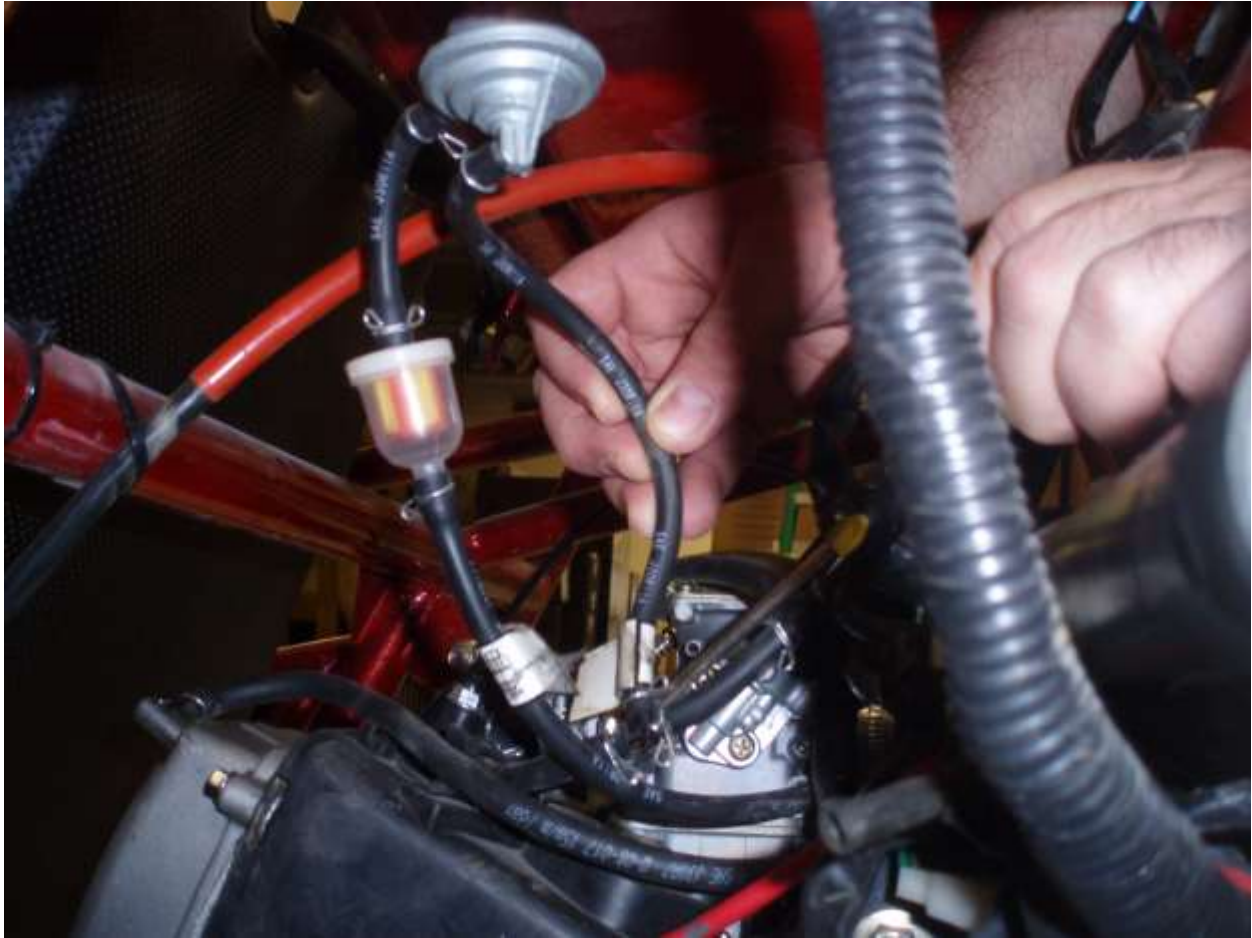
Figure 2: Vacuum line hookup.
