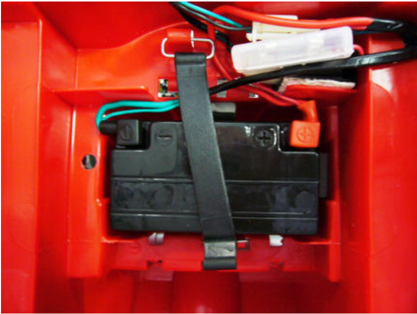
step13-fig2-Battery installation
