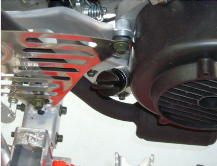
step19-fig2-Engine oil fill
