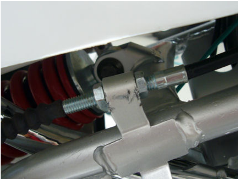
step15-fig3-Rear brake cable free play adjustment
