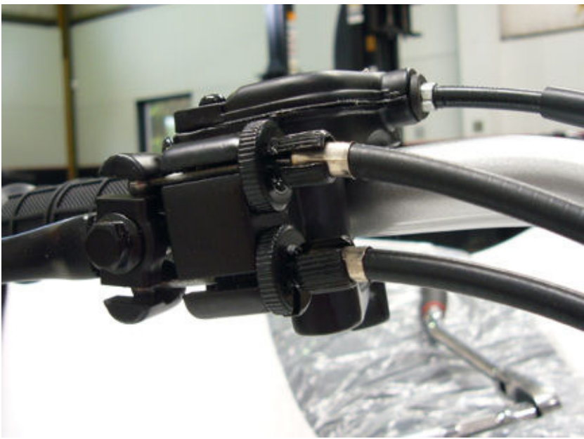
step15-fig2-Front brake cable free play adjustment
